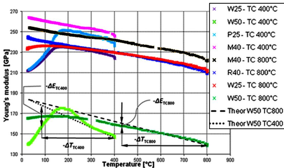
Figure A9. Young's moduli in temperature cycles RT-400°C and RT-800°C for \text{Al}_2\text{O}_3/\text{Cu} composites with different microstructures and copper contents. On the example of W50 IPC specimen, the idea of [191,192] is presented how to obtain curves showing differences between theoretical and real Young's moduli decrease upon cooling for two thermal cycles RT- 400°C and RT-800°C.
