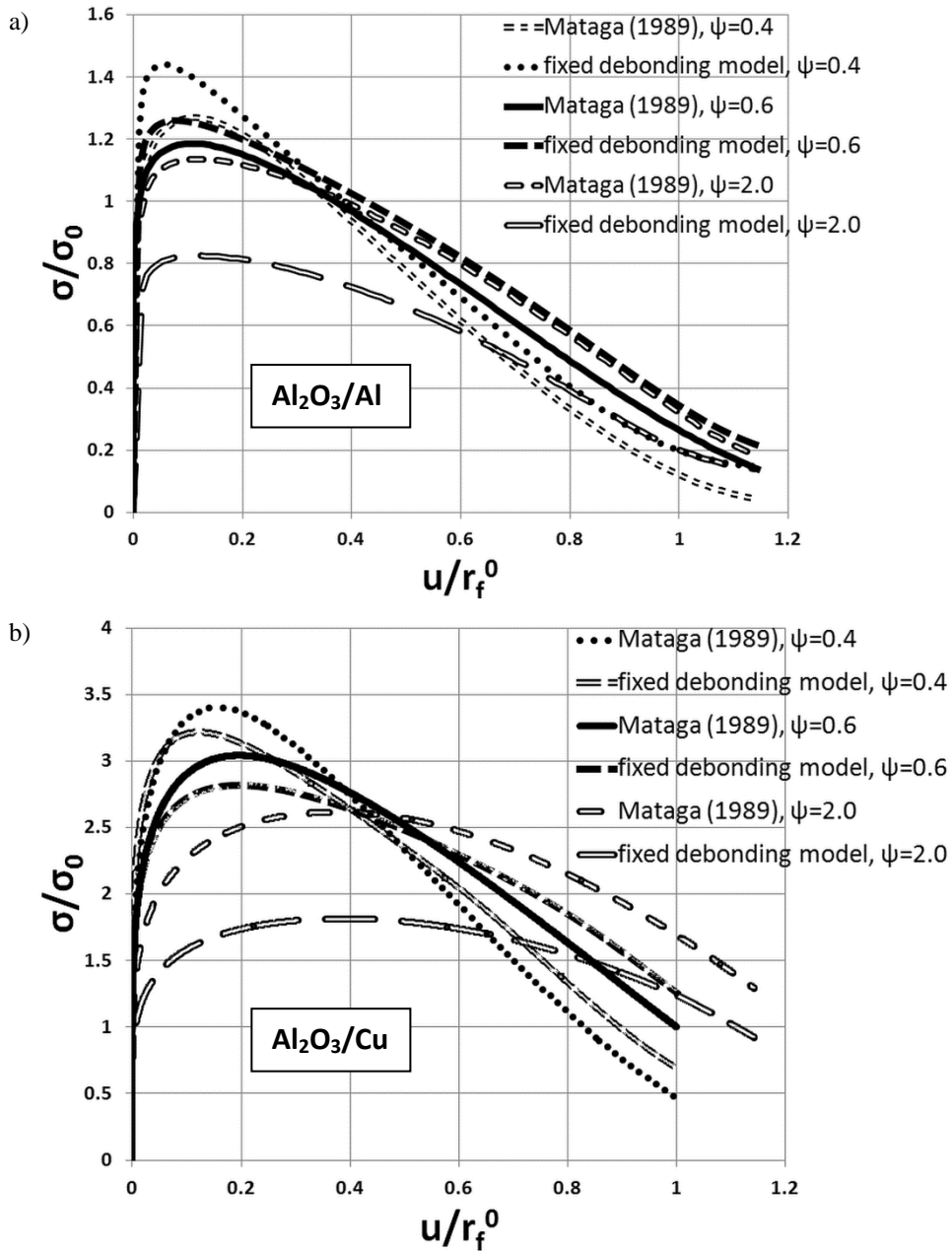
Figure 6.17. Normalized stress-displacement relationships in the reinforcing fibre from the numerical model with fixed debonding lengths, compared with the analytical solutions of [93] for different values of debonding parameter \psi : a) \text{Al}_2\text{O}_3/\text{Al} , b) \text{Al}_2\text{O}_3/\text{Cu} .
