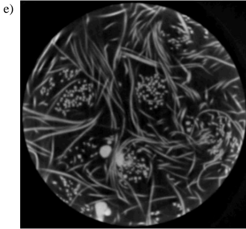
Figure A5. Microstructure of the infiltrated \text{Al}_2\text{O}_3/\text{Cu} IPC composites (micro-CT images, courtesy of G. Geier, Leoben):
