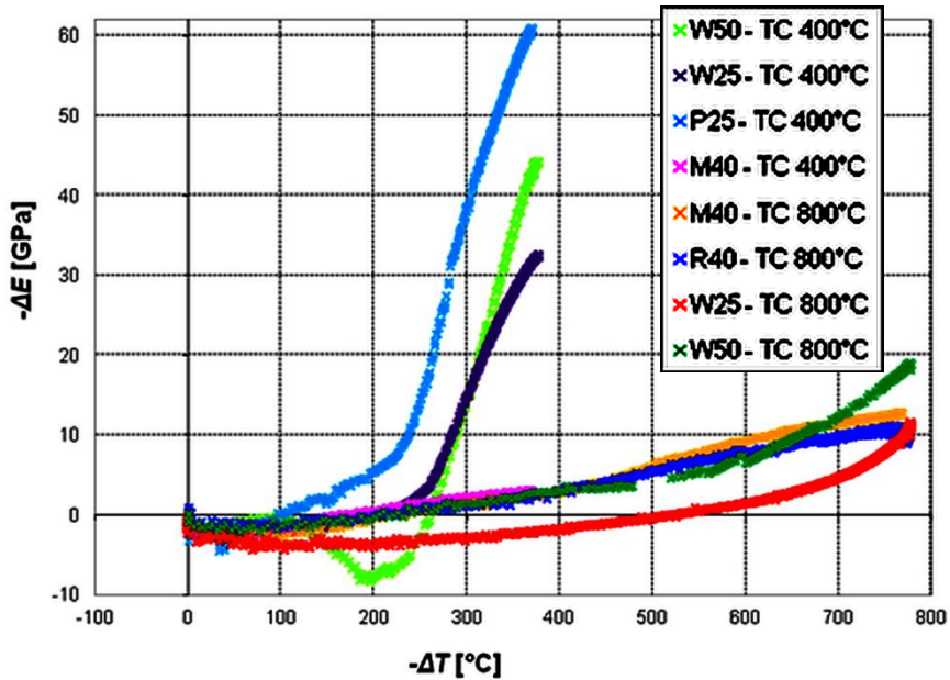
Figure A11. Reduction of Young's modulus vs. temperature decrease in cooling, temperature cycles up to 400°C and 800°C for \text{Al}_2\text{O}_3/\text{Cu} IPC composites with different microstructures and copper contents (the idea of the graph is explained in Figure A9).
