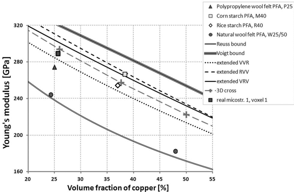
Figure A8. Effect of microstructure and copper content on \text{Al}_2\text{O}_3/\text{Cu} composites Young's moduli. Measurements done with Grindosonic impulse excitation of vibration equipment and compared with Voigt and Reuss bounds, extended V-V-R , R-V-V and V-R-V models and
