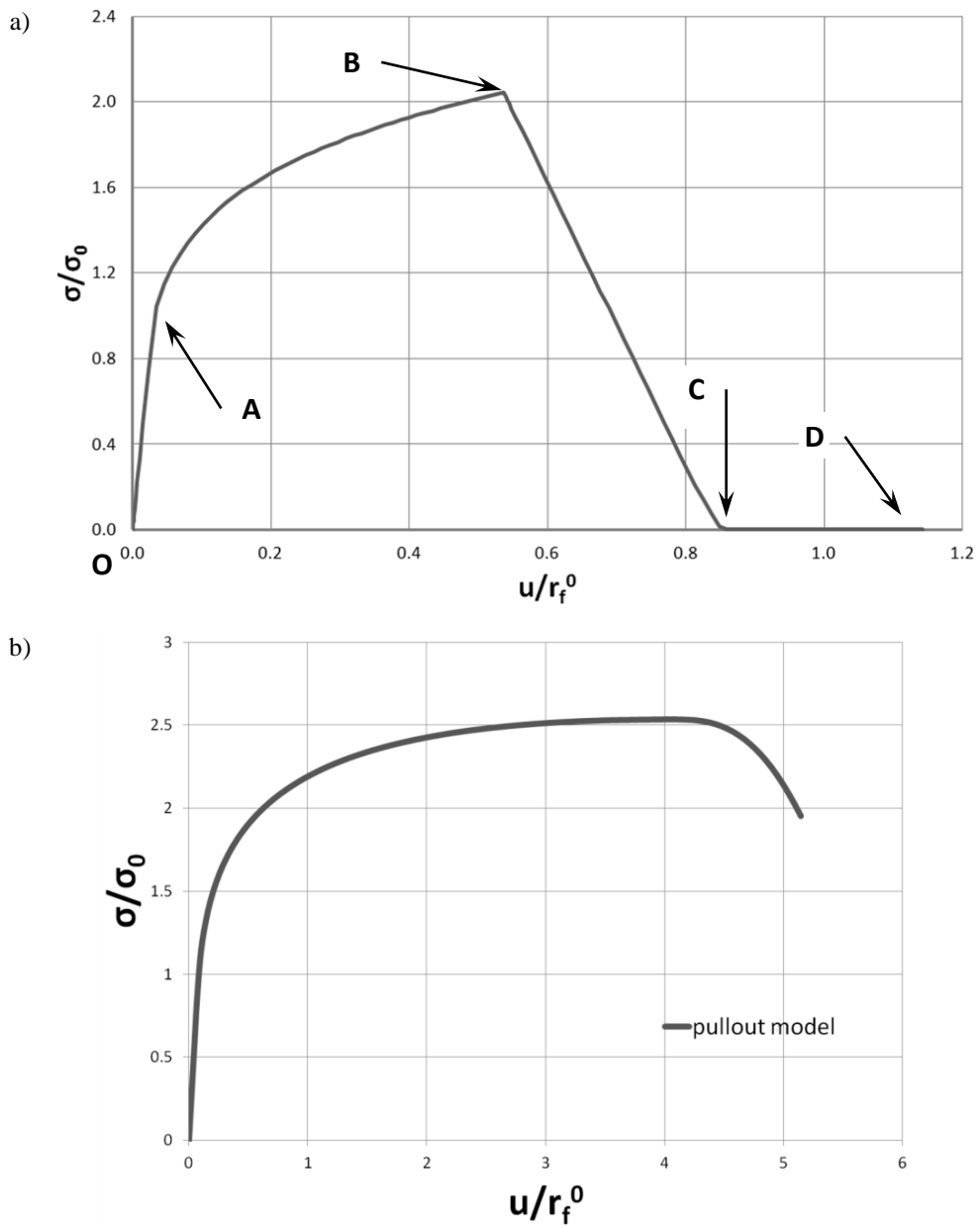
Figure 6.20. Normalised stress-displacement relationships obtained from present numerical model of the pullout problem; a) at debonding shear stress in the interface \tau_{\max,0} = 3.0 MPa with the main stages of the pullout process marked with letters O ÷ D , b) at parameters from Table 6.4.
