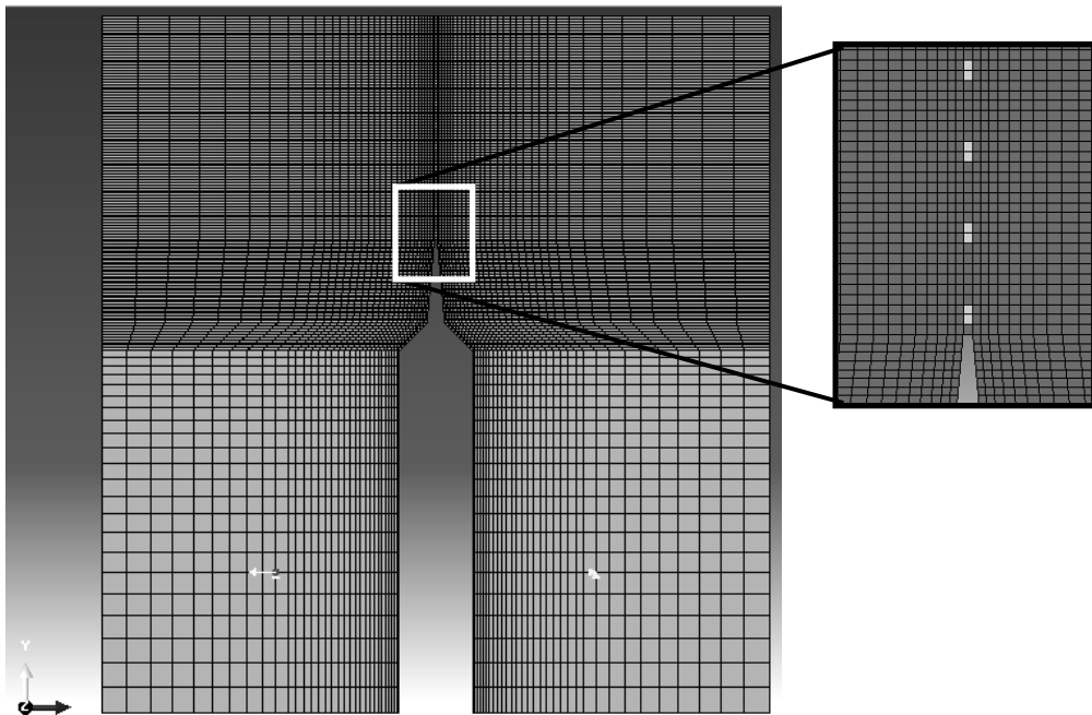
Figure 6.30. Compact-Tension (C-T) test model in ABAQUS [144] (mesh created with FEAP [156]) with bridging fibres modelled as plane strain elements (light colour), boundary conditions and displacement loading.
