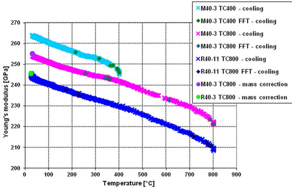
Figure A10. Young's modulus in temperature cycles for \text{Al}_2\text{O}_3/\text{Cu} IPCs based on corn and rice starch
