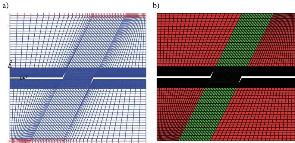
Figure 6.9. a) FEM mesh and boundary conditions, b) materials: red – \text{Al}_2\text{O}_3 , green – Cu
